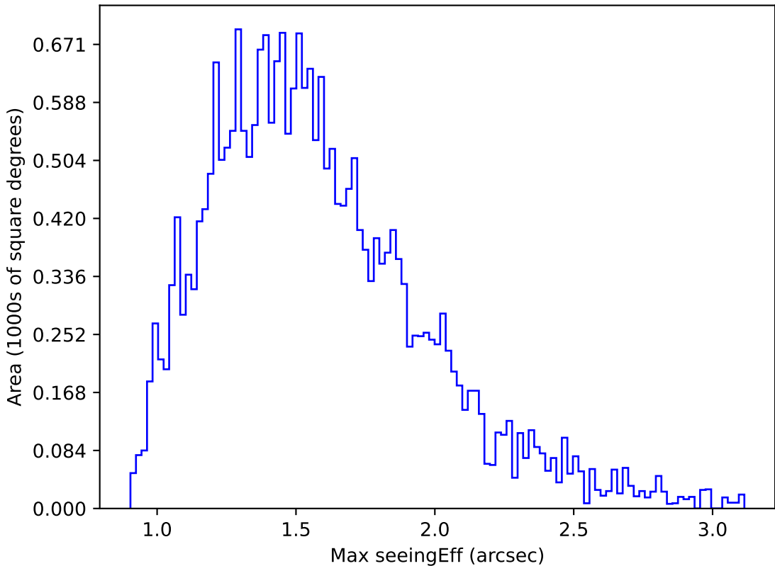
too_elab_r32_d2_griz_v3.4_10yrs Yr 1 g band: Max seeingEff
