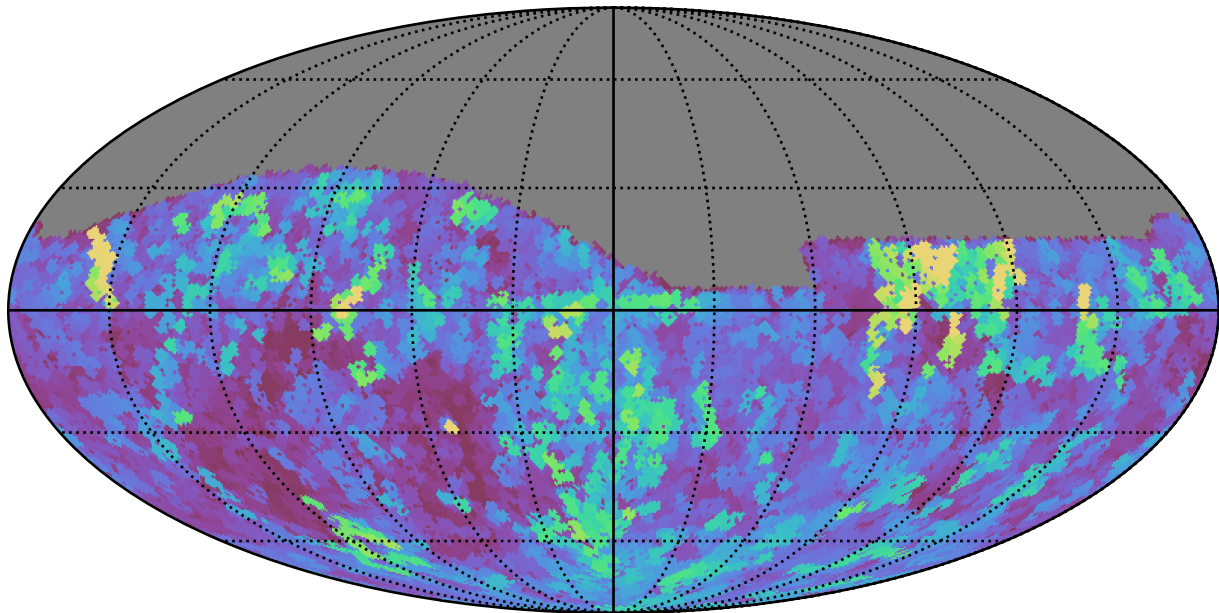
too_elab_r32_d2_griz_v3.4_10yrs Yr 1 all bands: Max seeingEff
