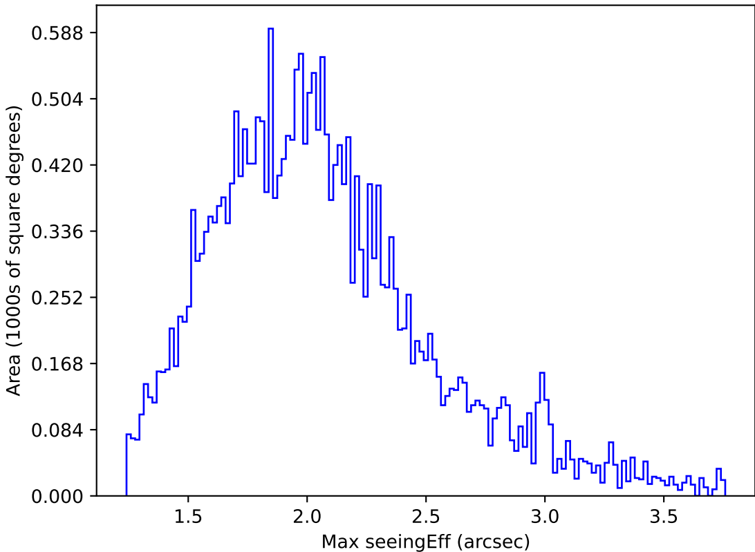
too_elab_r32_d2_griz_v3.4_10yrs Yr 1 all bands: Max seeingEff
