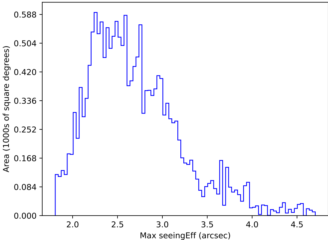
too_elab_r32_d2_griz_v3.4_10yrs WFD r band: Max seeingEff
