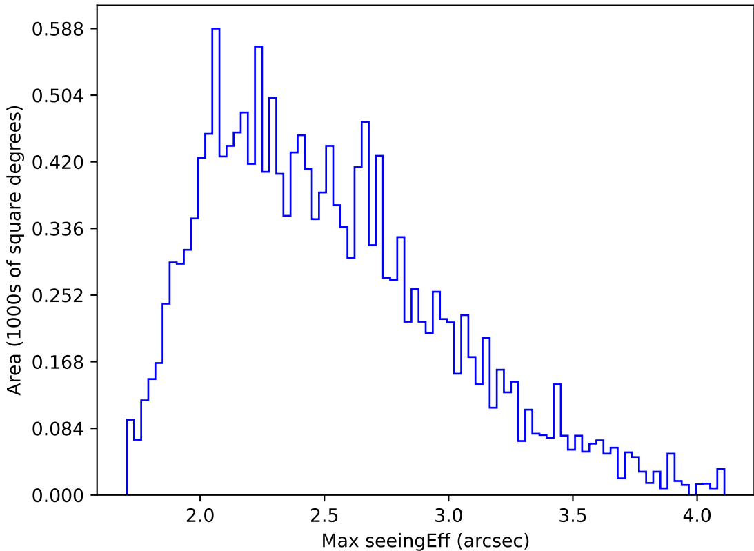
too_elab_r32_d2_griz_v3.4_10yrs WFD g band: Max seeingEff
