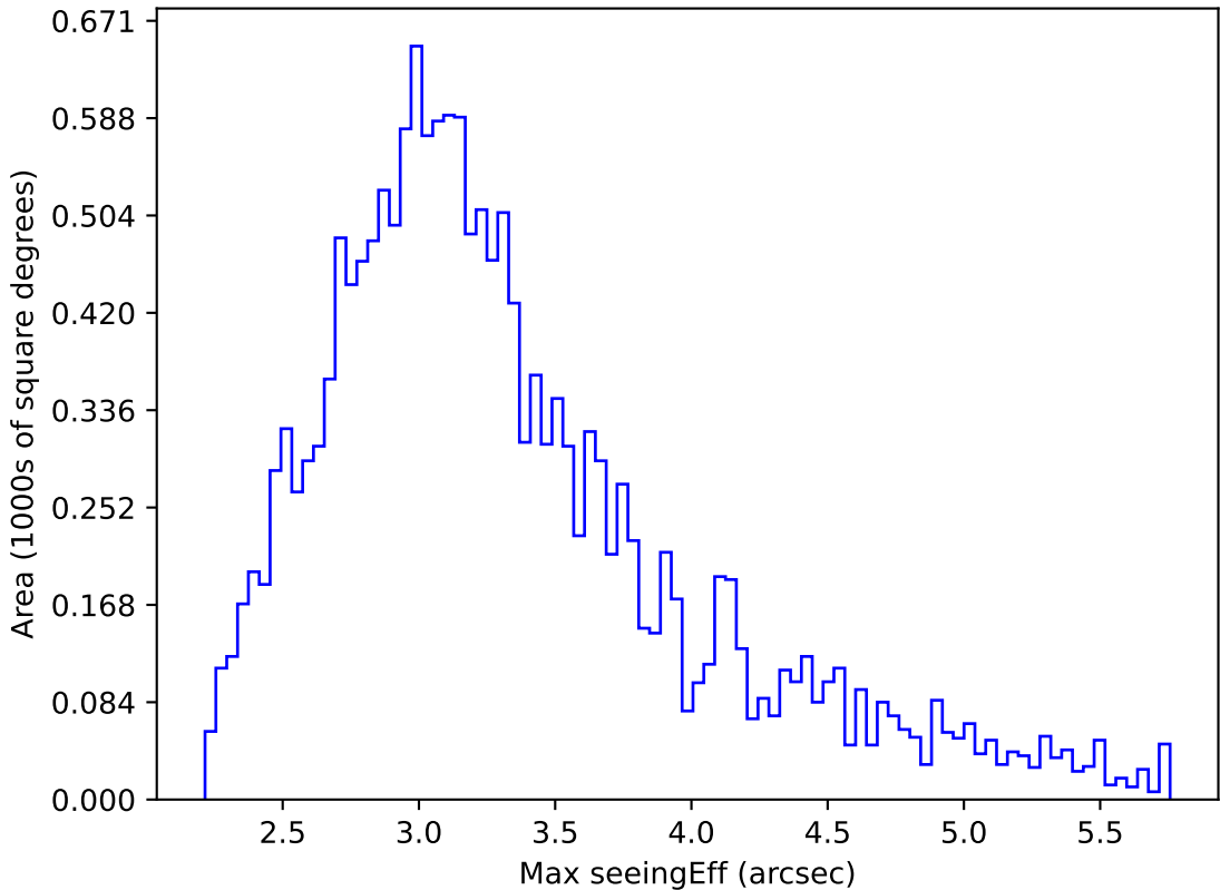
too_elab_r32_d2_griz_v3.4_10yrs WFD all bands: Max seeingEff
