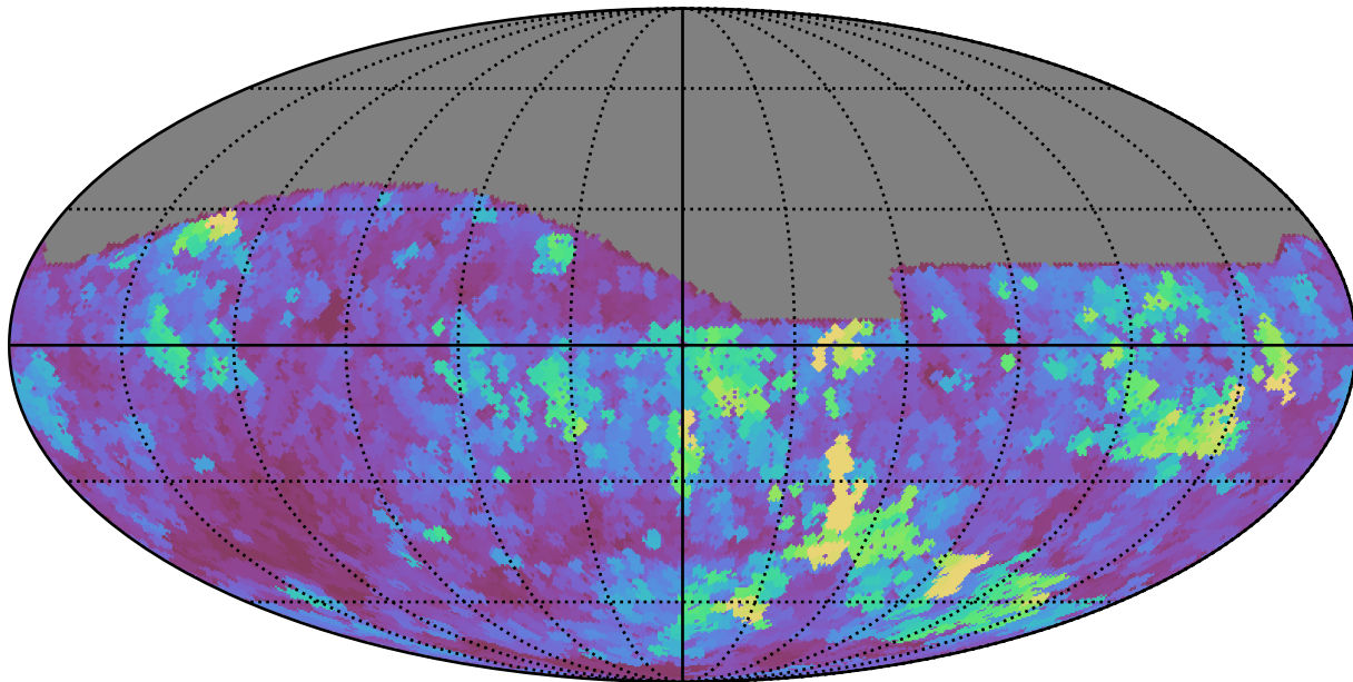
too_elab_r32_d2_griz_v3.4_10yrs All sky z band: Max seeingEff
