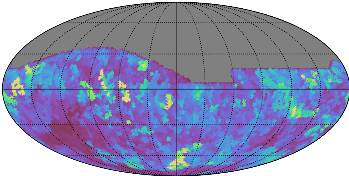
too_elab_r32_d2_griz_v3.4_10yrs All sky i band: Max seeingEff
