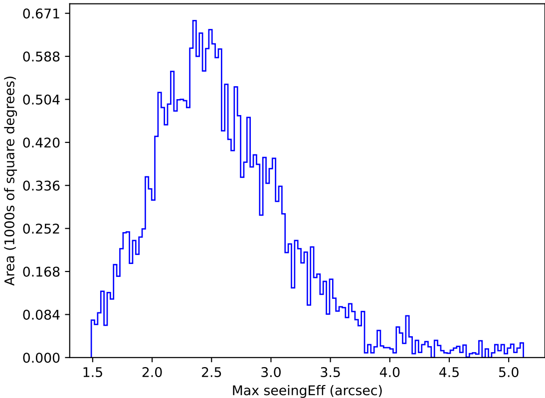
too_elab_r32_d2_griz_v3.4_10yrs All sky i band: Max seeingEff
