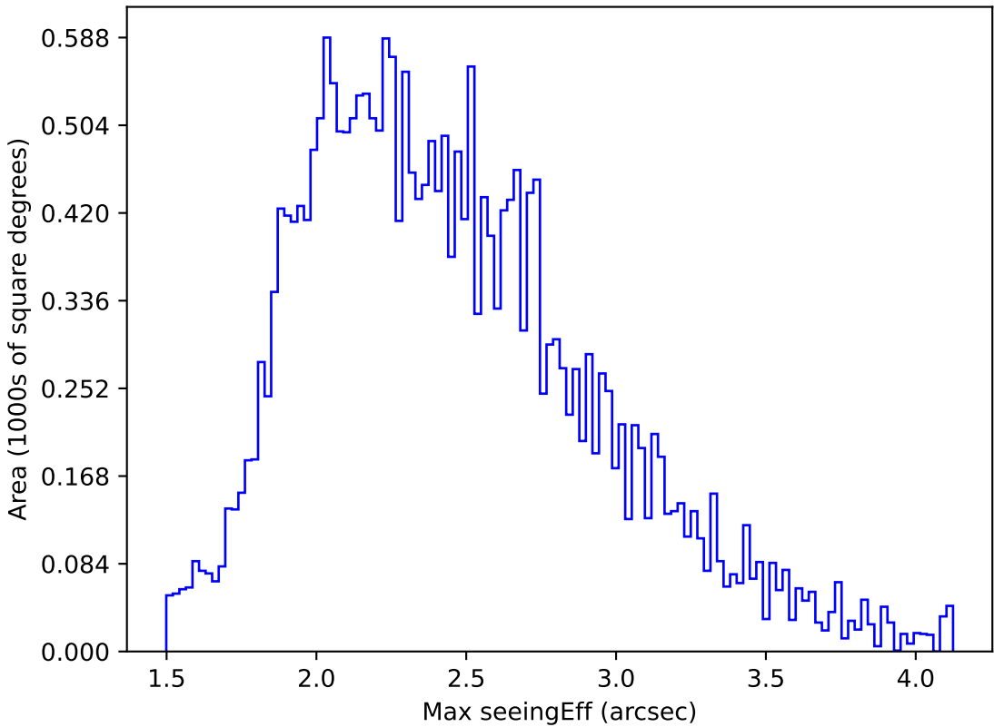
too_elab_r32_d2_griz_v3.4_10yrs All sky g band: Max seeingEff
