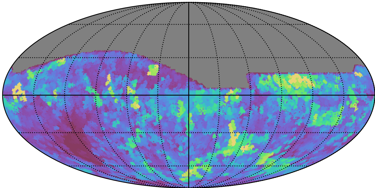
too_elab_r32_d2_griz_v3.4_10yrs All sky all bands: Max seeingEff
