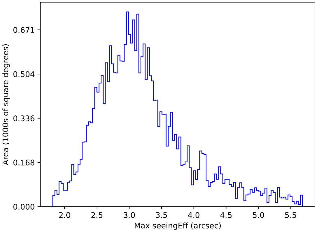
too_elab_r32_d2_griz_v3.4_10yrs All sky all bands: Max seeingEff
