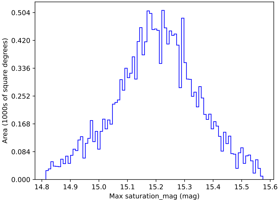
too_elab_r32_d2_griz_v3.4_10yrs WFD z band: Max saturation_mag
