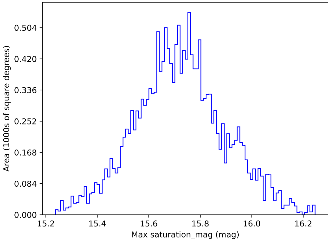
too_elab_r32_d2_griz_v3.4_10yrs WFD g band: Max saturation_mag
