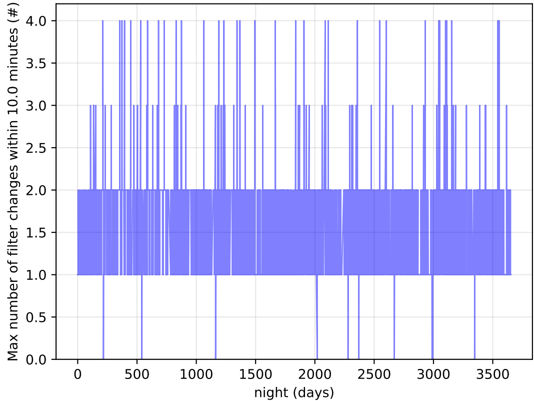
too_elab_r32_d2_griz_v3.4_10yrs Per Night: Max number of filter changes within 10.0 minutes
