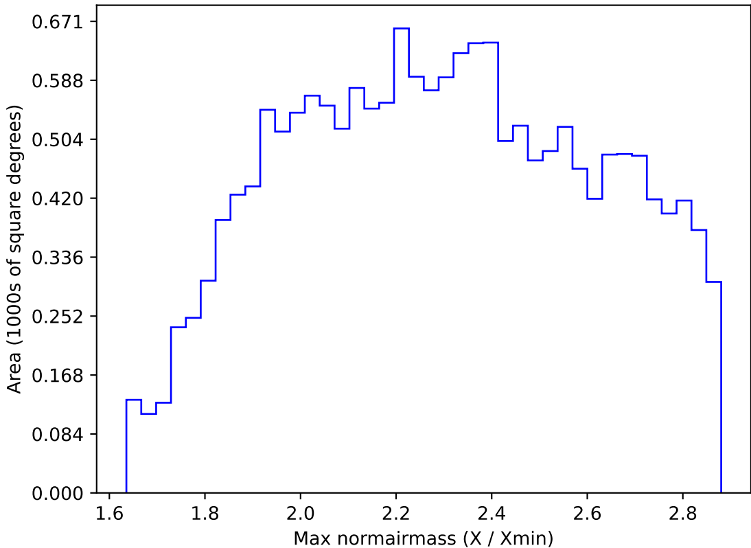
too_elab_r32_d2_griz_v3.4_10yrs WFD z band: Max normairmass
