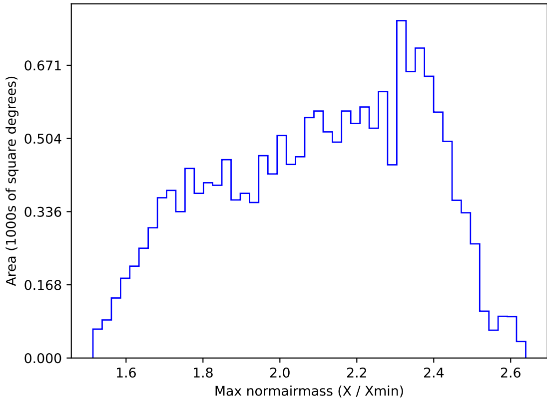
too_elab_r32_d2_griz_v3.4_10yrs WFD r band: Max normairmass
