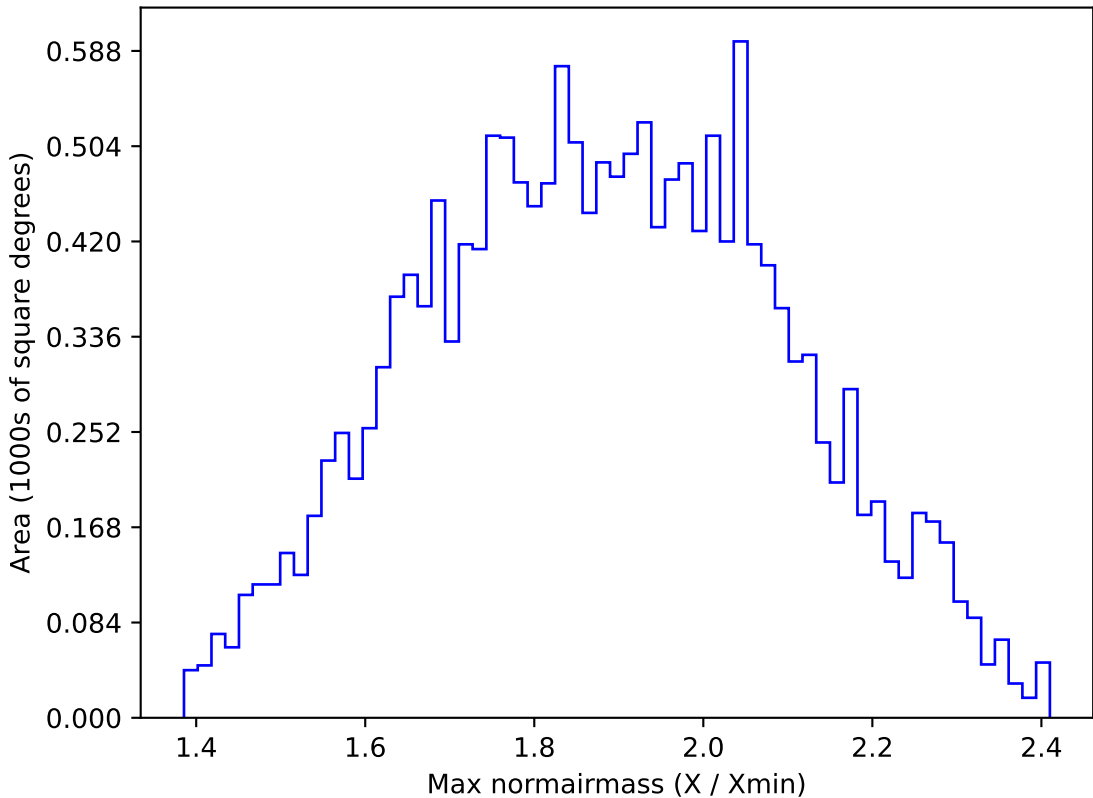
too_elab_r32_d2_griz_v3.4_10yrs WFD g band: Max normairmass
