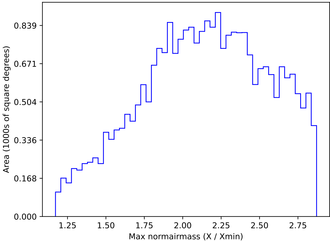
too_elab_r32_d2_griz_v3.4_10yrs All sky z band: Max normairmass
