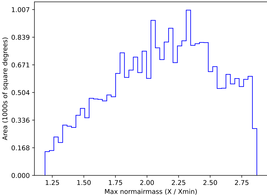
too_elab_r32_d2_griz_v3.4_10yrs All sky i band: Max normairmass
