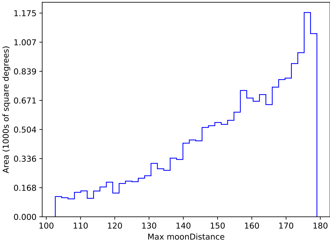
too_elab_r32_d2_griz_v3.4_10yrs WFD z band: Max moonDistance
