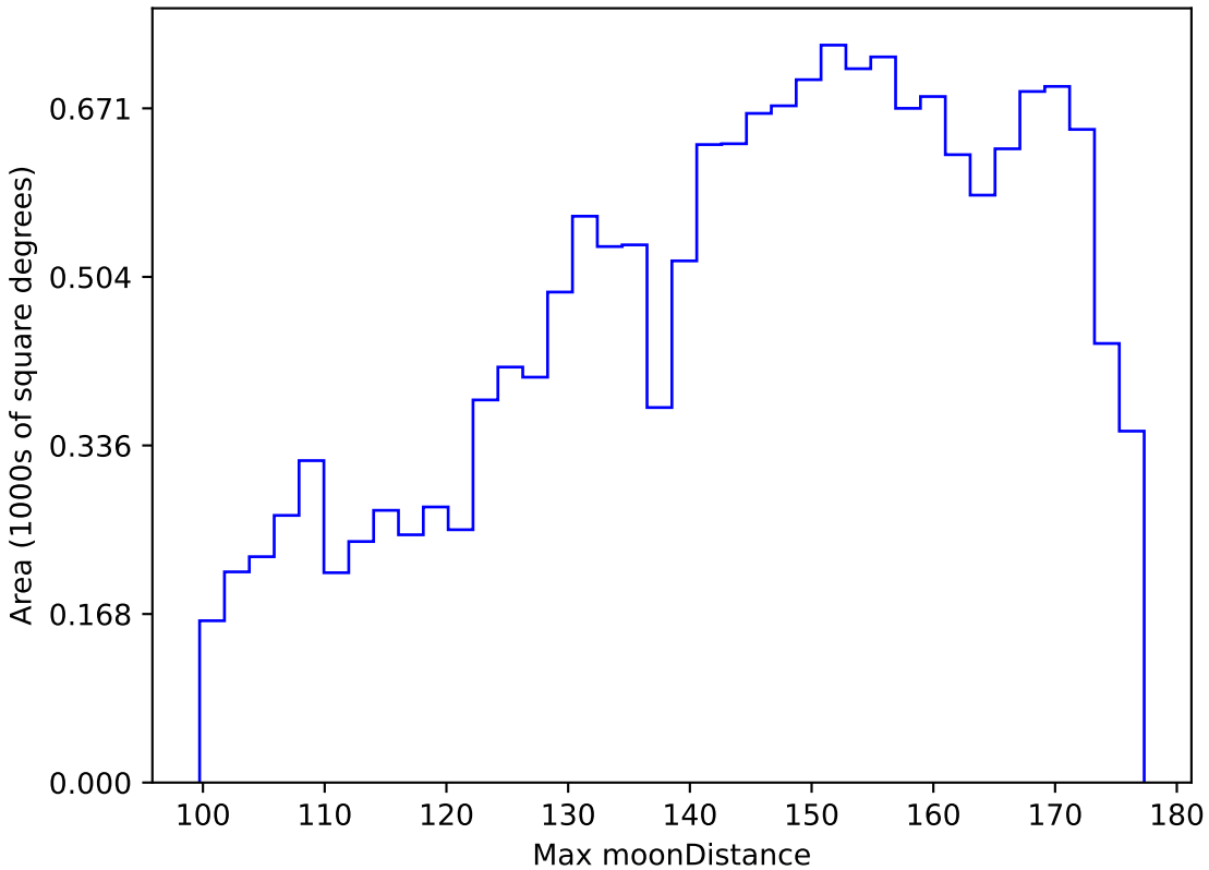
too_elab_r32_d2_griz_v3.4_10yrs WFD y band: Max moonDistance
