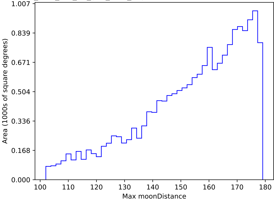
too_elab_r32_d2_griz_v3.4_10yrs WFD u band: Max moonDistance
