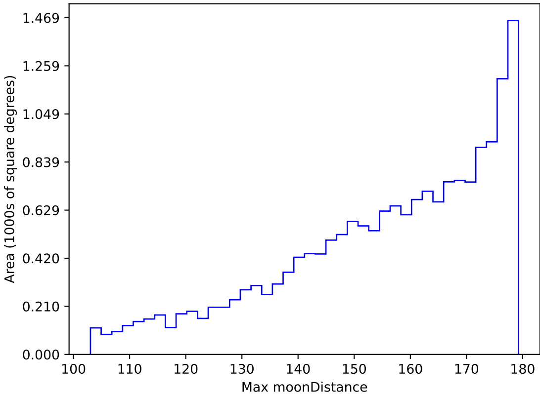
too_elab_r32_d2_griz_v3.4_10yrs WFD i band: Max moonDistance
