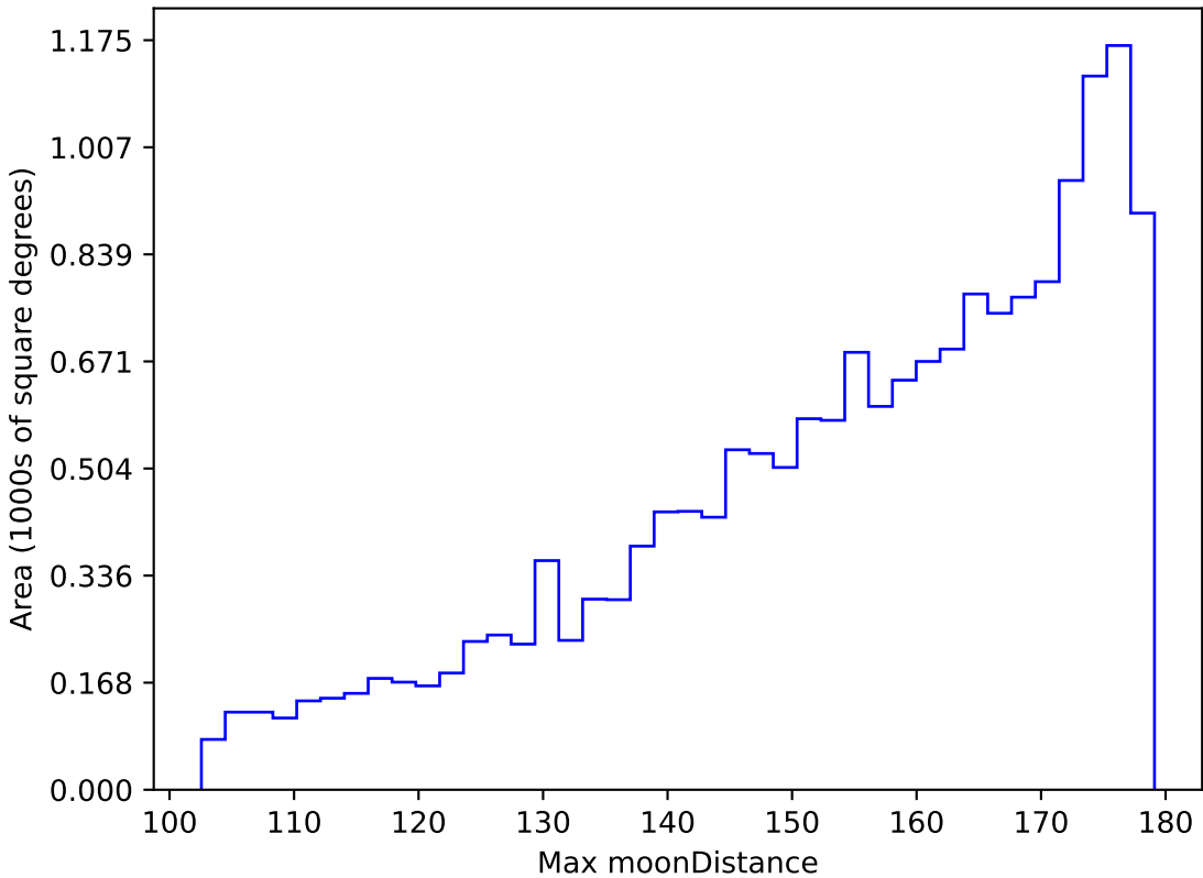
too_elab_r32_d2_griz_v3.4_10yrs WFD g band: Max moonDistance
