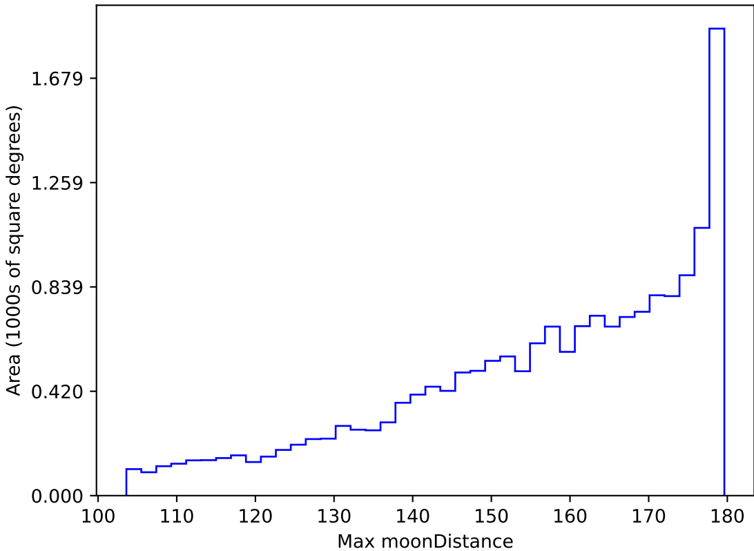
too_elab_r32_d2_griz_v3.4_10yrs WFD all bands: Max moonDistance
