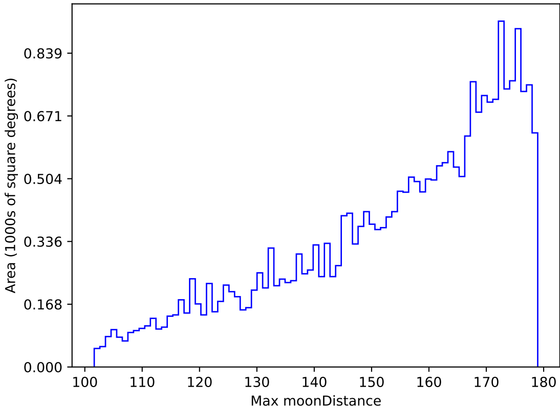
too_elab_r32_d2_griz_v3.4_10yrs All sky z band: Max moonDistance
