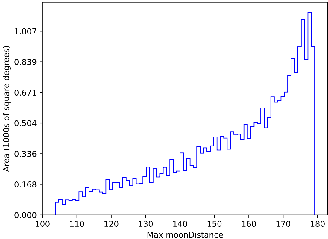
too_elab_r32_d2_griz_v3.4_10yrs All sky i band: Max moonDistance
