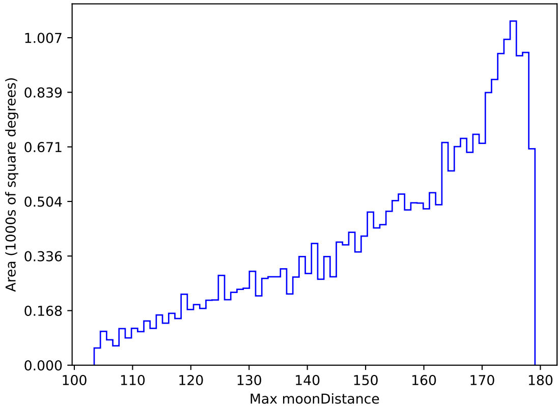
too_elab_r32_d2_griz_v3.4_10yrs All sky g band: Max moonDistance
