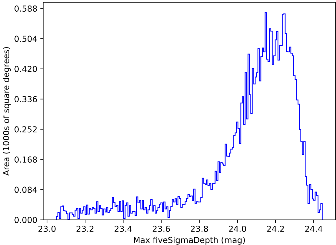
too_elab_r32_d2_griz_v3.4_10yrs Yr 1 i band: Max fiveSigmaDepth
