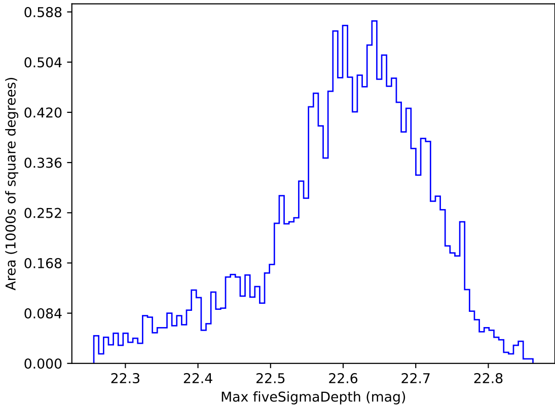
too_elab_r32_d2_griz_v3.4_10yrs WFD y band: Max fiveSigmaDepth
