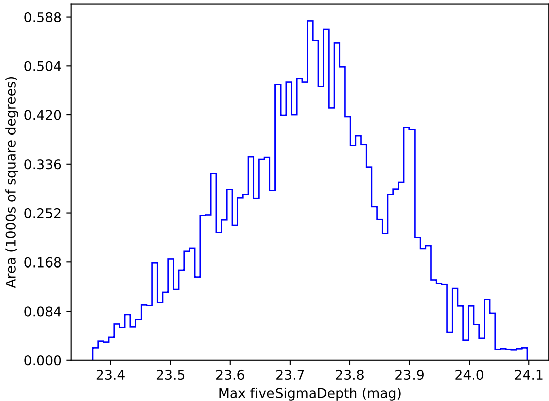
too_elab_r32_d2_griz_v3.4_10yrs WFD u band: Max fiveSigmaDepth
