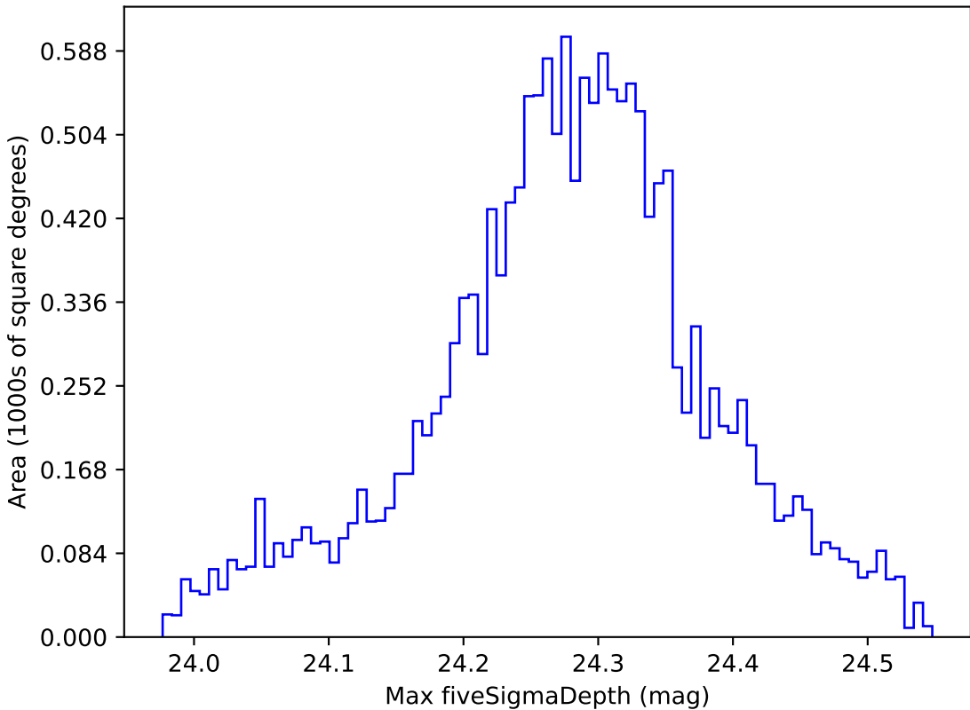
too_elab_r32_d2_griz_v3.4_10yrs WFD i band: Max fiveSigmaDepth
