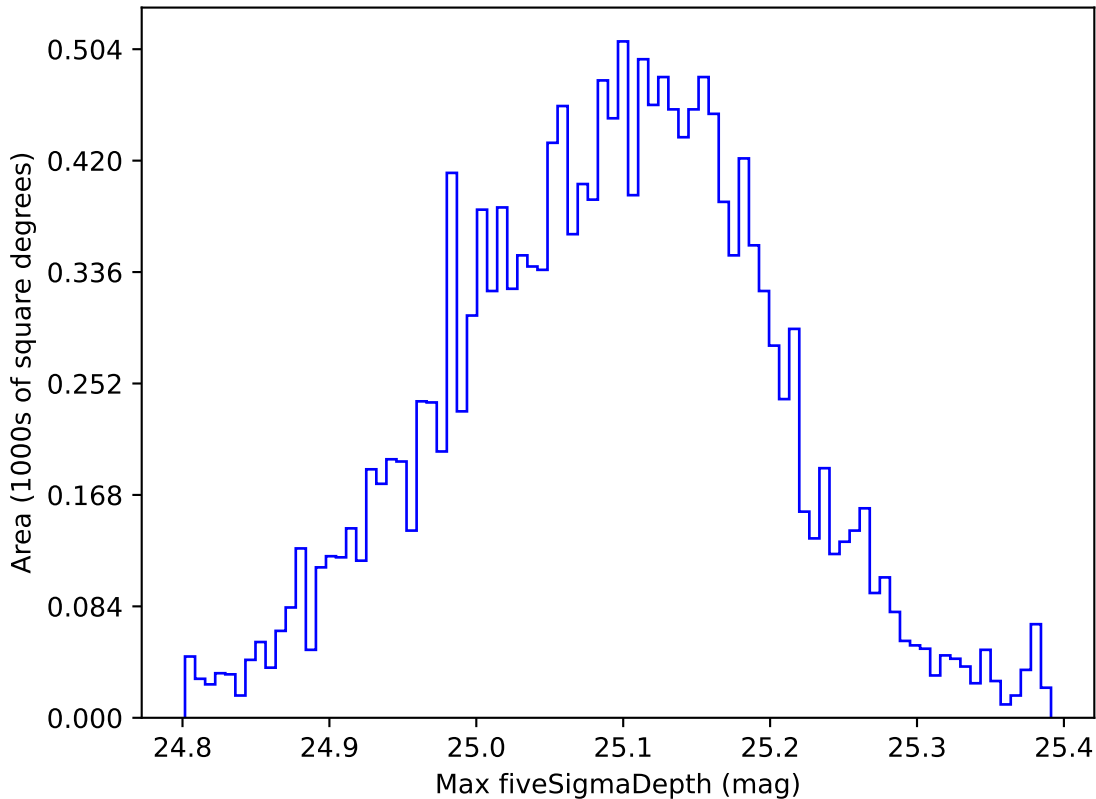
too_elab_r32_d2_griz_v3.4_10yrs WFD all bands: Max fiveSigmaDepth
