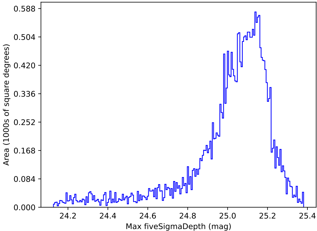
too_elab_r32_d2_griz_v3.4_10yrs All sky g band: Max fiveSigmaDepth
