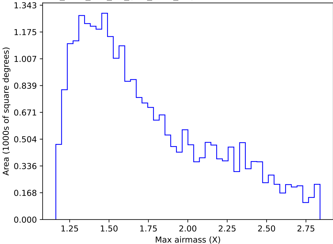
too_elab_r32_d2_griz_v3.4_10yrs Yr 1 z band: Max airmass
