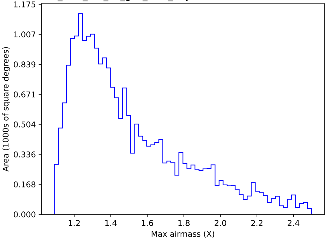
too_elab_r32_d2_griz_v3.4_10yrs Yr 1 u band: Max airmass
