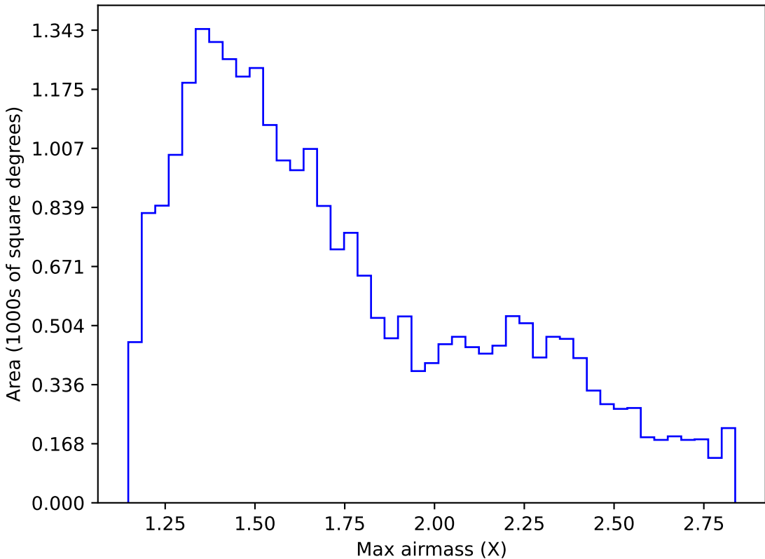
too_elab_r32_d2_griz_v3.4_10yrs Yr 1 i band: Max airmass
