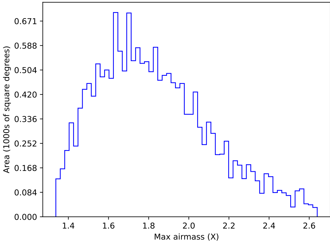
too_elab_r32_d2_griz_v3.4_10yrs WFD u band: Max airmass
