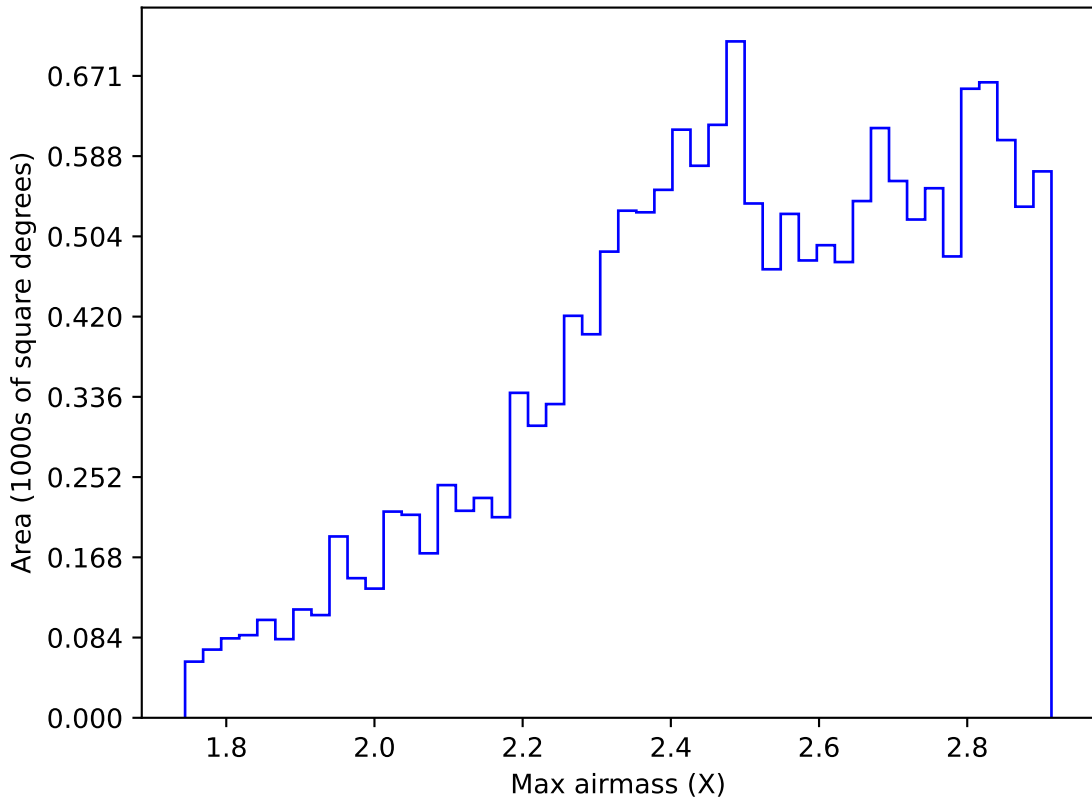
too_elab_r32_d2_griz_v3.4_10yrs WFD i band: Max airmass
