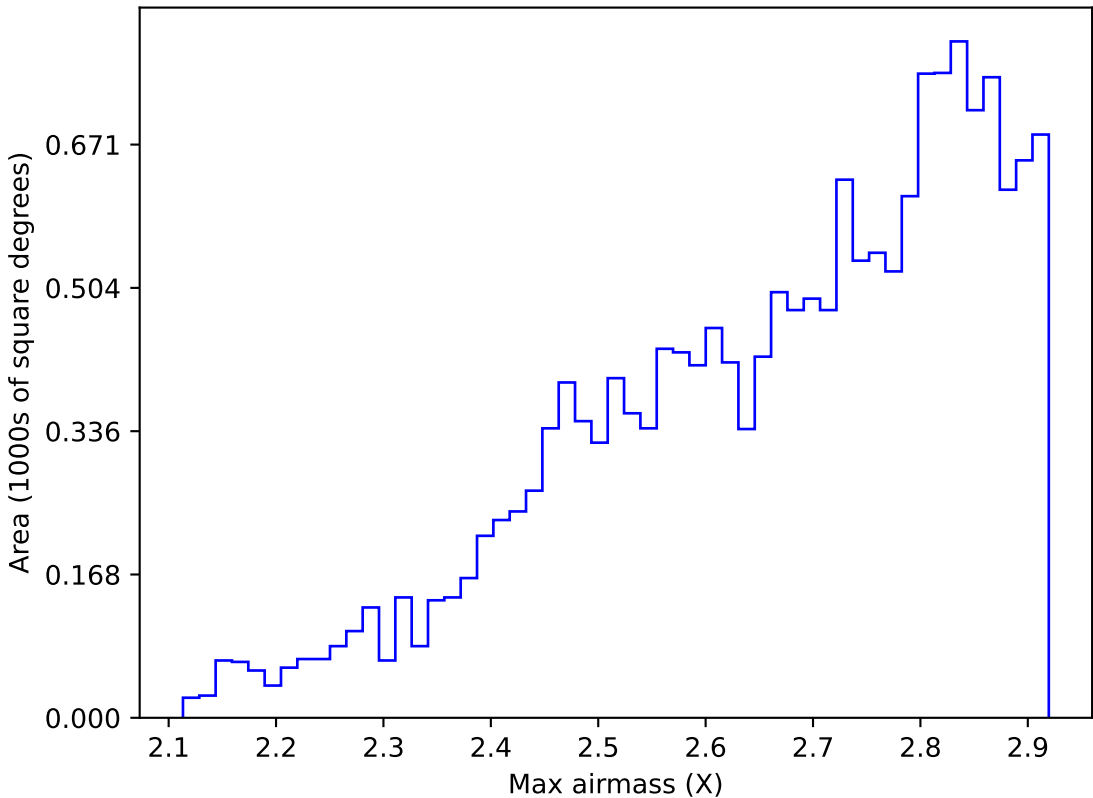
too_elab_r32_d2_griz_v3.4_10yrs WFD all bands: Max airmass
