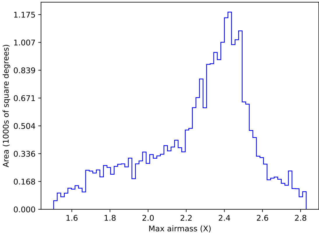
too_elab_r32_d2_griz_v3.4_10yrs All sky r band: Max airmass
