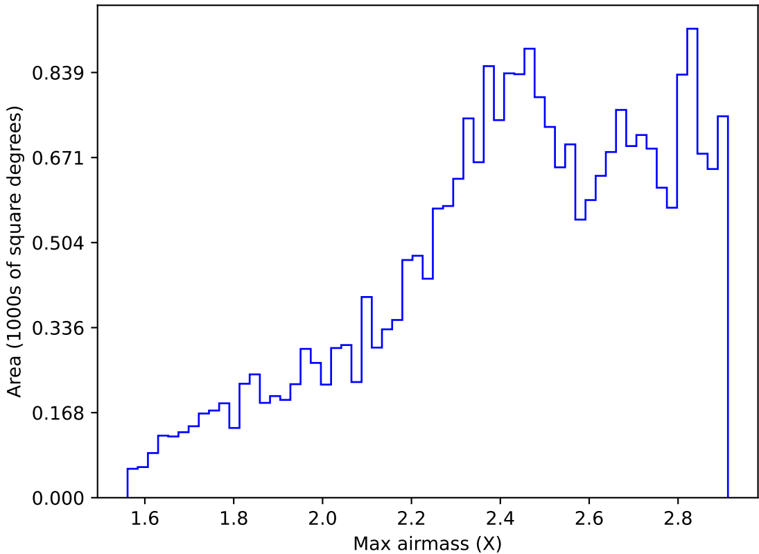
too_elab_r32_d2_griz_v3.4_10yrs All sky i band: Max airmass
