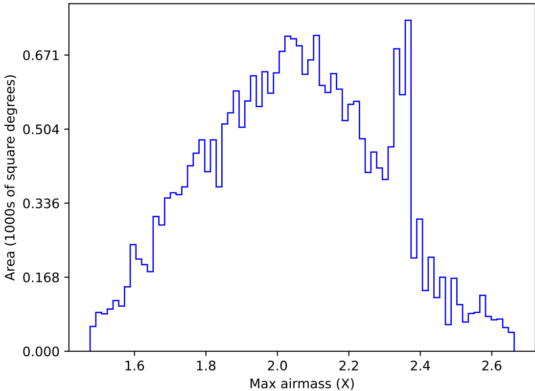
too_elab_r32_d2_griz_v3.4_10yrs All sky g band: Max airmass
