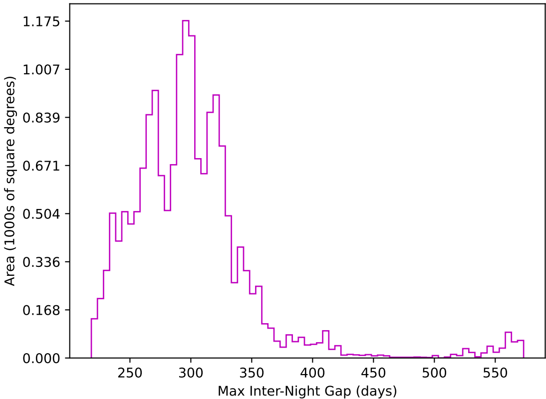
too_elab_r32_d2_griz_v3.4_10yrs WFD z band: Max Inter-Night Gap
