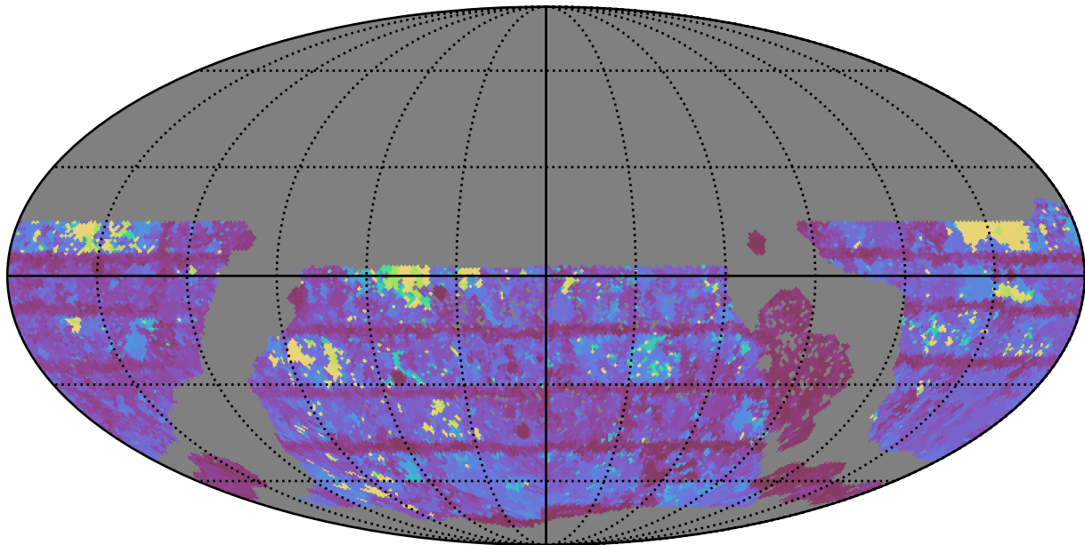
too_elab_r32_d2_griz_v3.4_10yrs WFD i band: Max Inter-Night Gap
