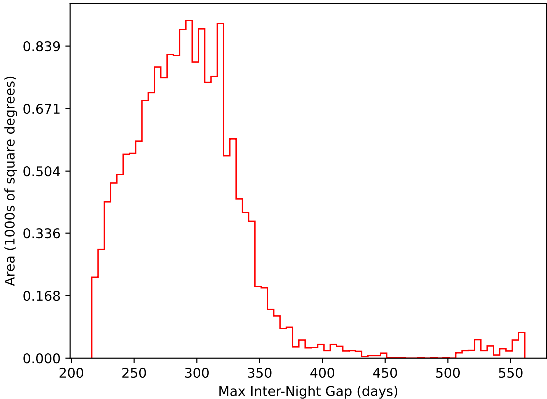
too_elab_r32_d2_griz_v3.4_10yrs WFD i band: Max Inter-Night Gap
