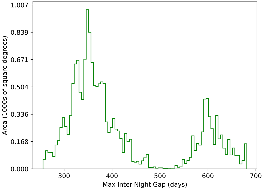
too_elab_r32_d2_griz_v3.4_10yrs WFD g band: Max Inter-Night Gap
