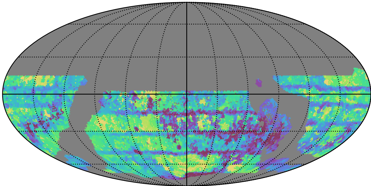
too_elab_r32_d2_griz_v3.4_10yrs WFD all bands: Max Inter-Night Gap
