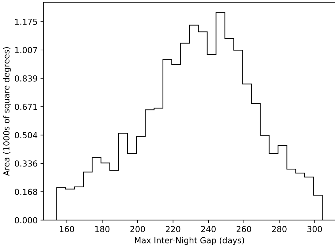
too_elab_r32_d2_griz_v3.4_10yrs WFD all bands: Max Inter-Night Gap
